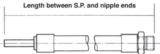
Straight standpipe
