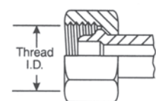
Female Universal 24° or 60° Cone
